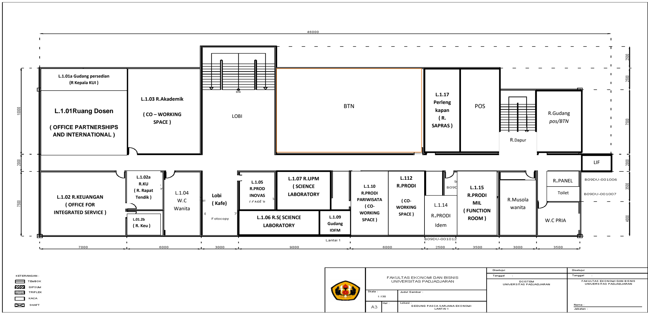
DENAH LT 1
